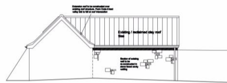
Side elevation
