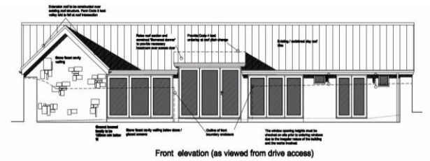
Front elevation (as viewed from drive access)
